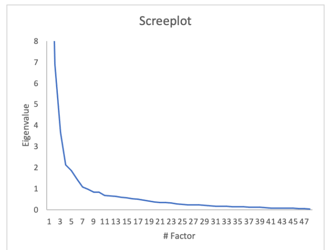
Fig. 2. Screeplot showing the number of factors
